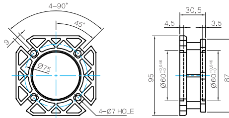
● MODEL: WHG-040-F
