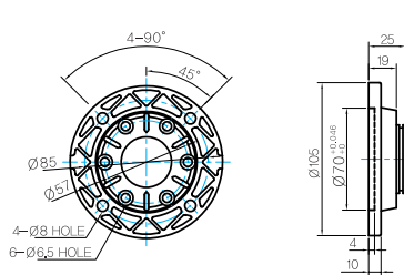
● MODEL: 040-Flange-71B14
