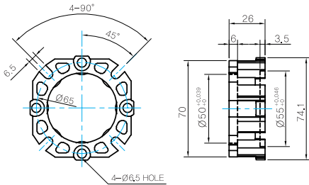
● MODEL: WHG-030-F
